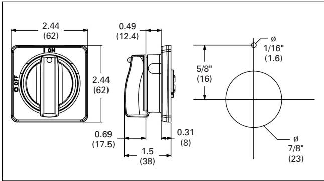
Figure 11. Selector Handle
